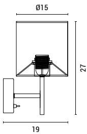
144-31035 AENON 52023933 Beige Metal-Pampas grass 1xE27 Max 40W 220-240V ø 190mm H: 270mm
