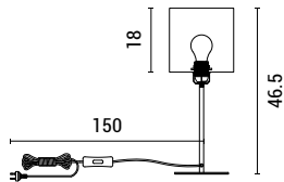
144-31033 AENON 52025382 Pampas Grass Metal-Pampas grass 1xE27 Max 40W 220-240V W: 180mm H: 465mm
