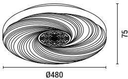
144-51038 TRIANO 52025624 White Plastic-Metal LED 60W 5700Lm 220-240V 3CCT(3000-4000-6000K) ø 480mm H: 75mm
