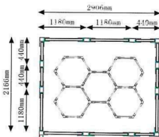
MODEL: AG-LG-310W
